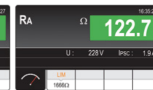
Measurement of overall earth resistance.
